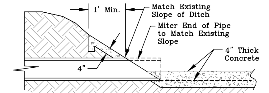
Sloped End Treatment - Profile N.T.S.
