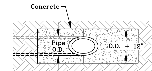
Sloped End Treatment - Plan N.T.S.
