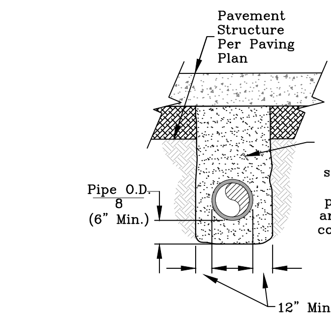
Bedding and Trench Backfill for PVC Pipe - Structural Areas N.T.S.
