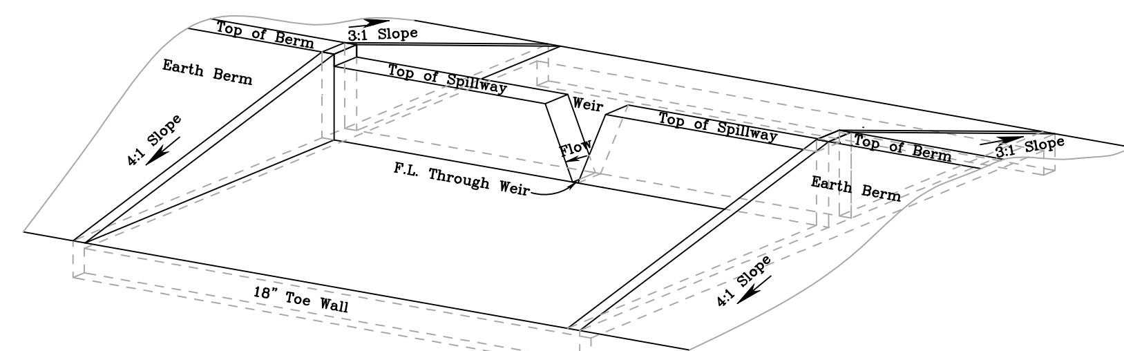
Detention Pond Outfall Structure: V-Notch Weir N.T.S.
