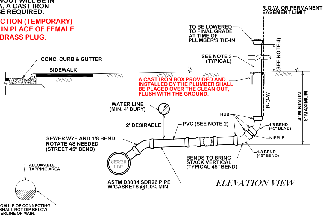
STANDARD SEWER SERVICE CONNECTION NEW CONSTRUCTION ONLY S6-00
